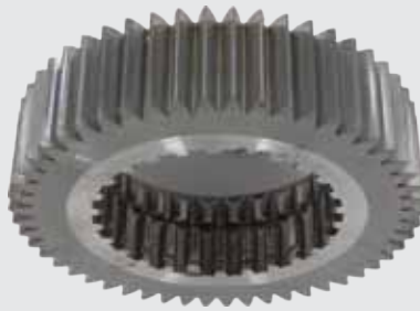
The transmission's mainshaft input drive gear demonstrated no pitting or scoring despite 512,000 miles of rigorous use. The gear earned a high wear rating of 8 out of 10, indicating only trace-light wear.
