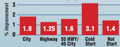
SAE 5W-40 Fuel Economy Results - FTP Cycle Fuel Economy Improvement
